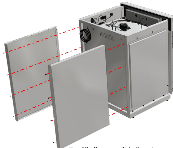
Fig. 32: Remove Side Panels
