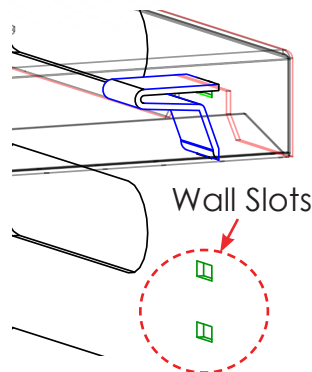
Fig. 18: Support Clip Fitted in Notch
