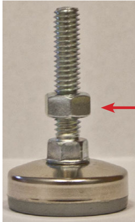
Fig. 7: Leg Leveler
