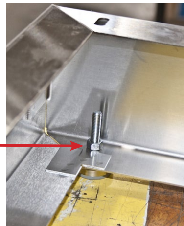
Fig. 11: Leg Leveler - Incorrect installation
