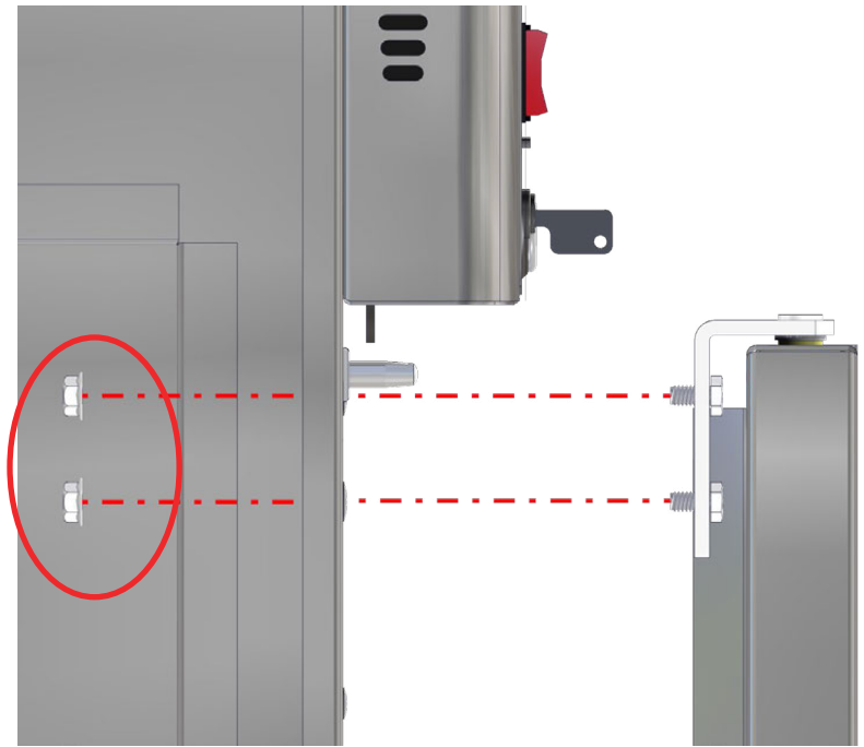
Fig. 68: Install Top Hinge and Secure Door
