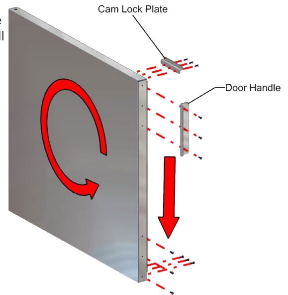
Fig. 64: Move Door Handle and Cam Lock Plate
