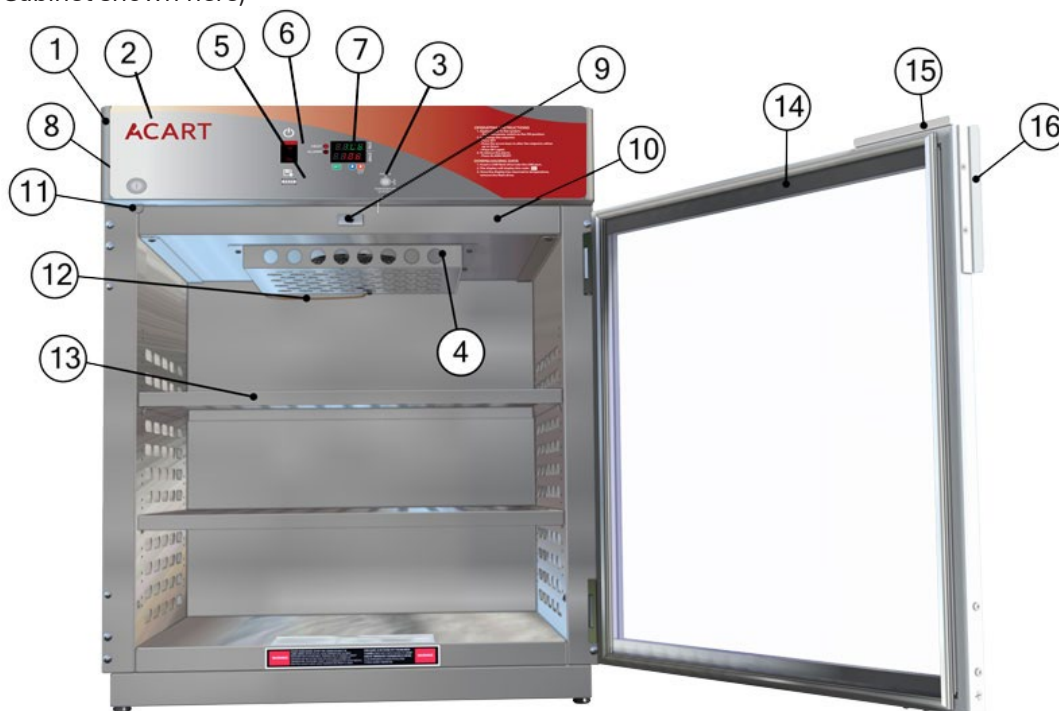
Fig. 5: Main Elements of Warming Cabinet
